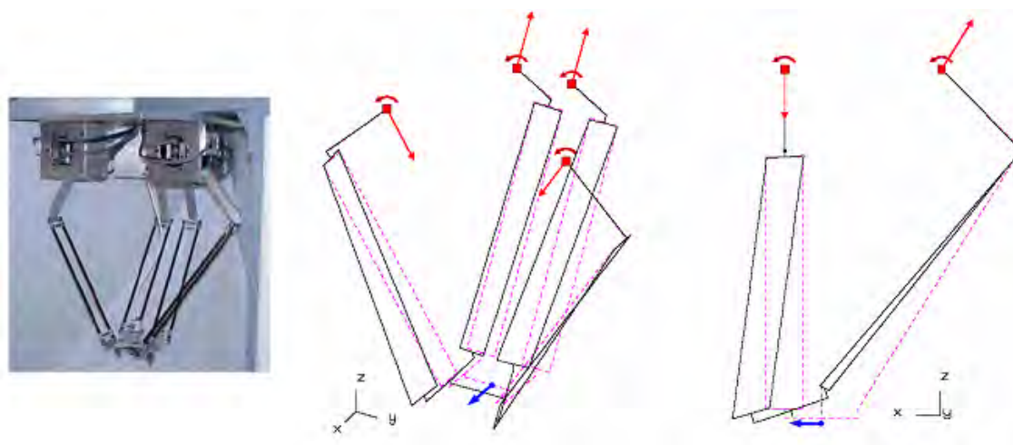
Figure 2. (a) Prototype of H4 robot; (b) FEA model of H4 robot (Corradine et al., 2004).
