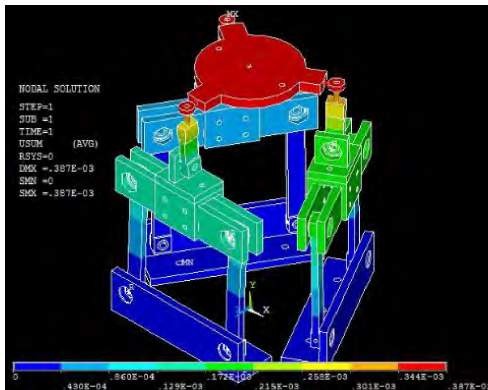
Figure 6. FEA model results of the CaPaMan-2bis when applied the loads F_x = F_y = F_z = 100N .
