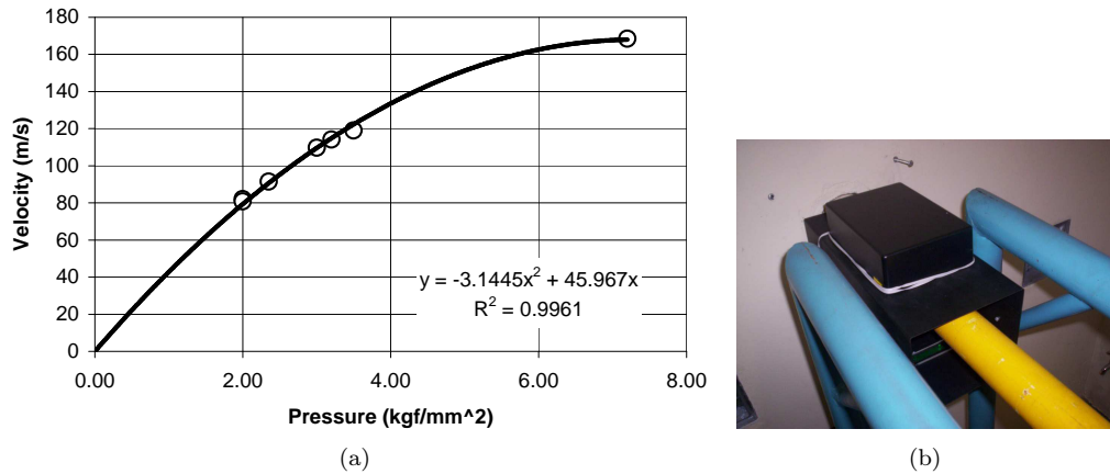
Figure 2: (a) Pressure versus velocity for the gas gun with bore diameter of 50mm. (b) Infra-red velocimeter.
