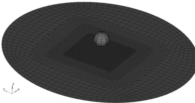
Figure 9: Final finite shell element mesh used in the analysis. The solid element mesh was extruded from this one.
