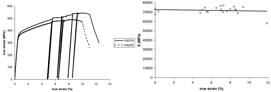
Figure 5: (a) Unidimensional true stress–strain curve for the aluminium alloy. (b) Elastic modulus degradation under tensile loading.
