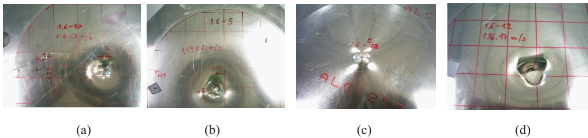
Figure 4: Plate hit by a hard sphere at impact velocities of (a) V_0 = 116.03\text{m/s} , (b) V_0 = 119.02\text{m/s} , (c) V_0 = 117.37\text{m/s} and (d) V_0 = 136.17\text{ m/s} .
