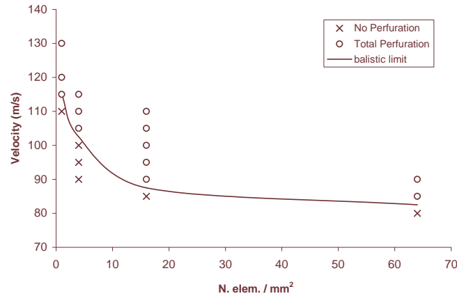
Figure 8: Influence of the mesh density on the ballistic limit.
