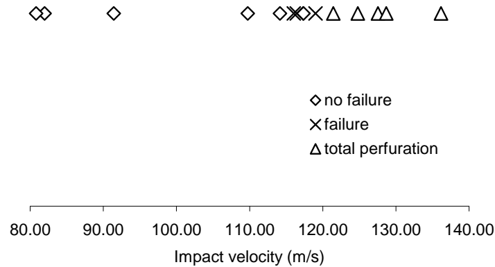
Figure 3: Plate response to the impact velocity.
