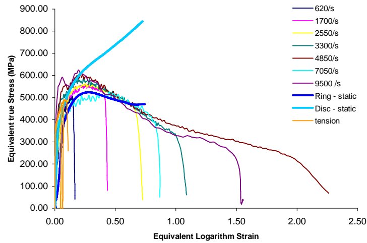
Figure 7: Stress–strain behaviour at various strain rates and room temperature.
