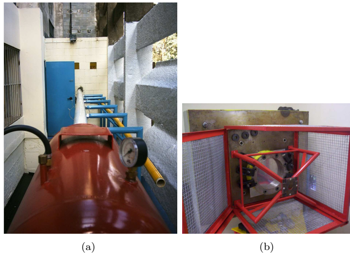
Figure 1: (a) Overview of the projectile launcher. (b) Protection chamber for the tests.
