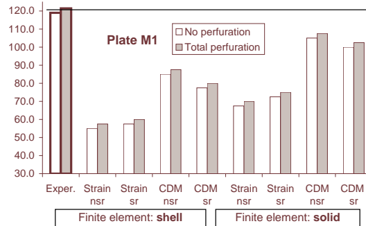
Figure 10: Ballistic limit for the aluminium plate according to the failure criteria. ( nsr ), sr – (non)-strain-rate sensitive, respectively.
