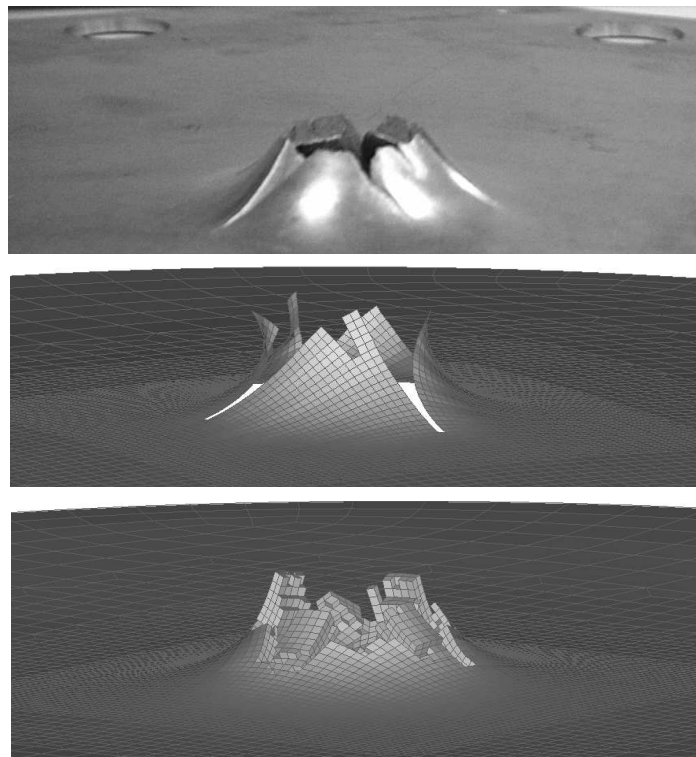
Figure 11: Fracture in an impacted plate and a shell plus solid finite element model.
