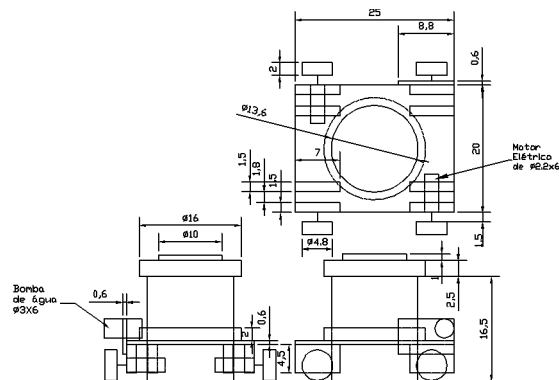
Figure 13. Top view, right side view and front view of the vehicle.
