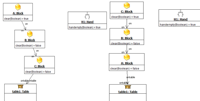
Figure 5. Initial and Final Snapshot of the planning problem related with Blocks World .
