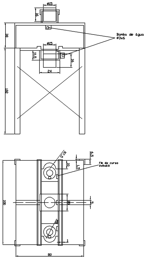
Figure 12. Front view and top view of the bench.
