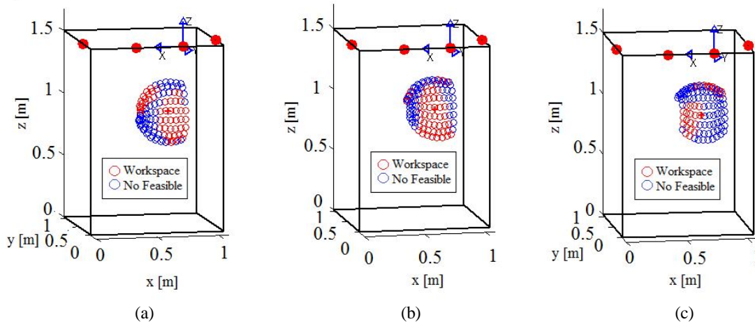
Figure 13. (a) Workspace with \gamma = -50^\circ (rotation z ) constant; (b) Workspace with \gamma = 0^\circ (rotation z ) constant; (c) Workspace with \gamma = 50^\circ (rotation z ) constant
