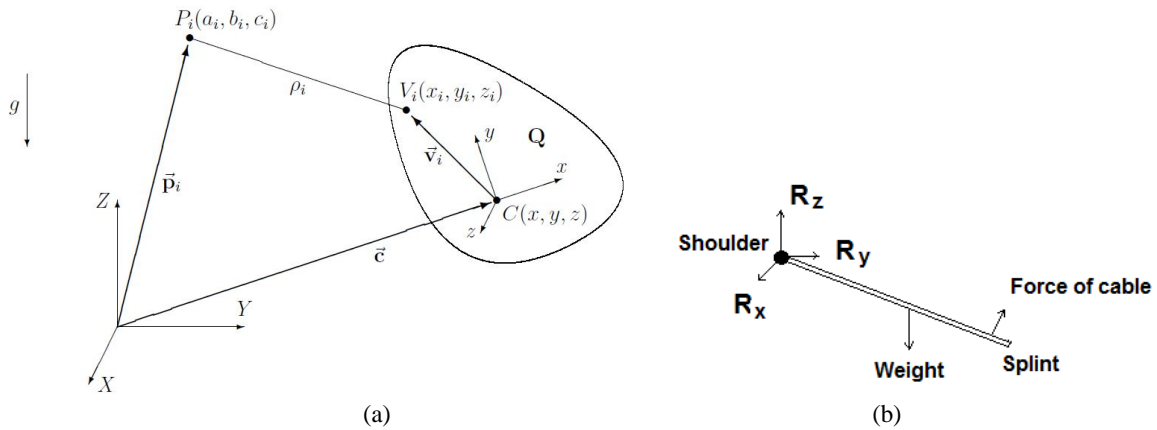
Figure 5. (a) Kinematic variables (Côté, 2003); (b) A scheme for a cable-based parallel architecture proposed
