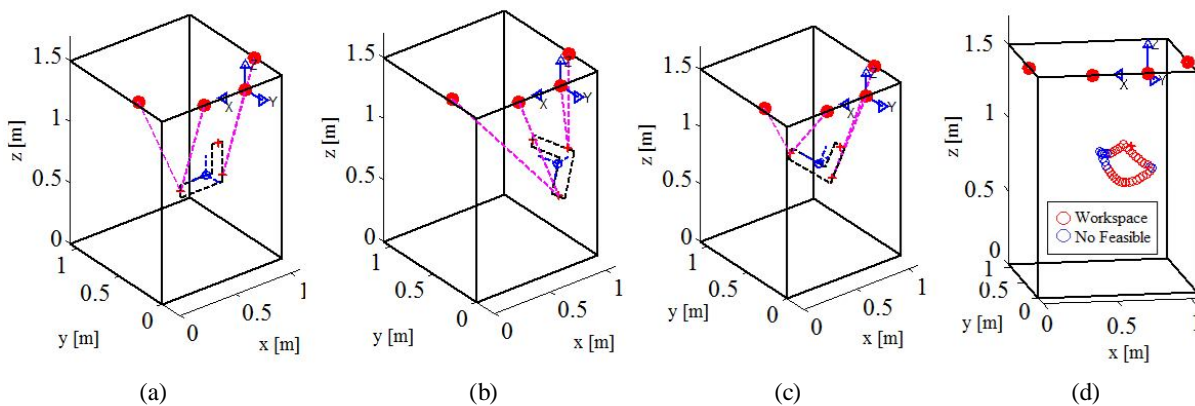
Figure 12. (a) Splint the initial position 0^\circ ; (b) Rotation in x ( 45^\circ ) and y ( 50^\circ ); (c) Rotation in x ( 45^\circ ) and y ( -50^\circ ); (d) Workspace.
