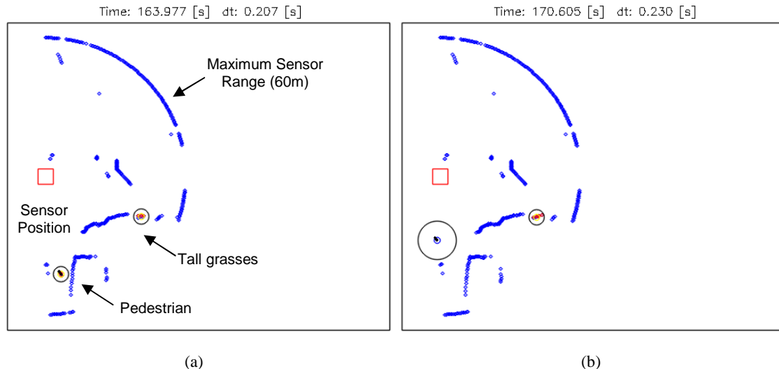
Figure 7: Tracking Obstacles and Predicting their Future States. In (a) a pedestrian is tracked inside the sensor range, and in (b), the tracker is kept even while the pedestrian is out of the sensor range.
