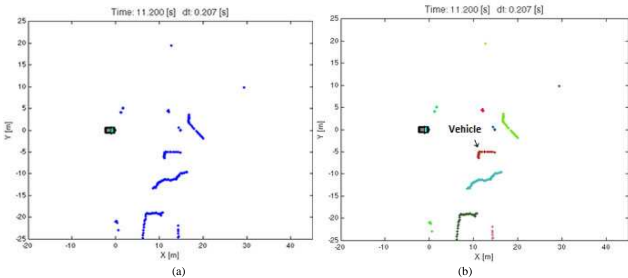
Figure 4: Results obtained during the segmentation process. In (a): environment data acquired by the laser sensor (the blue dots represent the obstacles detected). In (b): the output of the segmentation procedure algorithm (each obstacle is represented by a different color - in detail, a vehicle that was detected).
