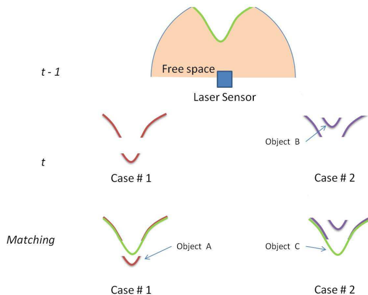
Figure 2: Illustration of the rules proposed by Wang and Thorpe (2002) for obstacle detection. Wang and Thorpe (2002) presented in their work an obstacle detection method based on two rules:
