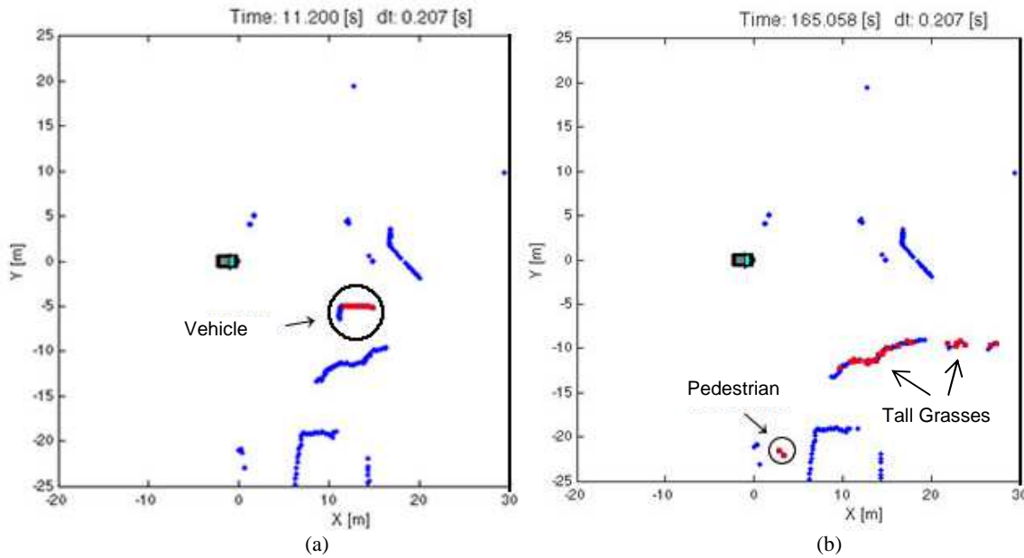
Figure 6: Results of the algorithm for obstacle detection.
