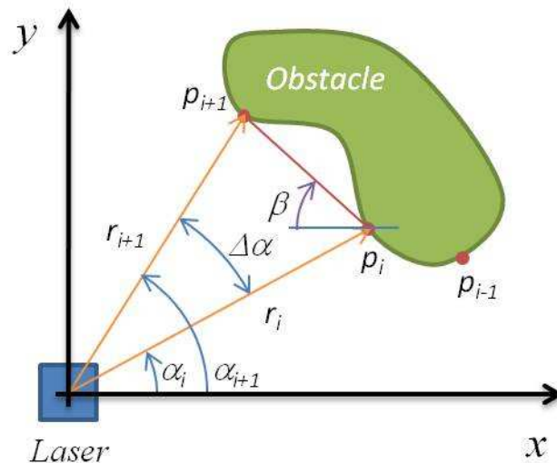
Figure 1: Representation of the laser readings and some of its parameters used on the segmentation procedure. In this figure, p_{i-1}, p_i, p_{i+1} represent a sequence of laser readings.
