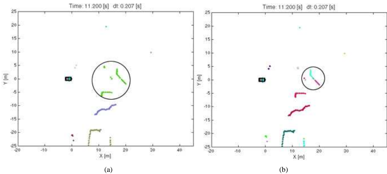
Figure 5: Results obtained during the segmentation process for two different values of the threshold distance between the laser data. In (a): the segmentation algorithm fused several objects into a single one (green dots inside the black circle). In (b): the segmentation algorithm divided a single object into two distinct ones (blue and violet dots inside the black circle).
