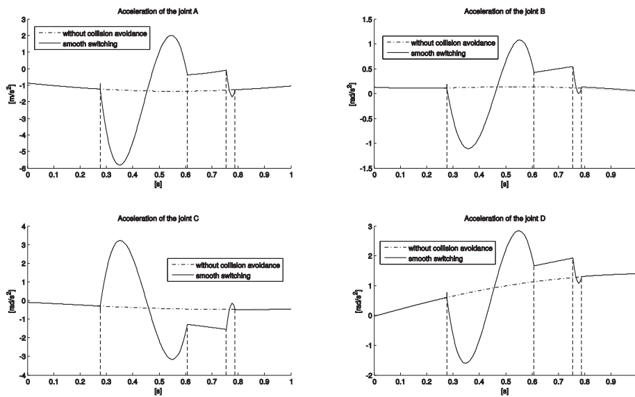
Figure 5. Accelerations of the joints A , B , C and D
