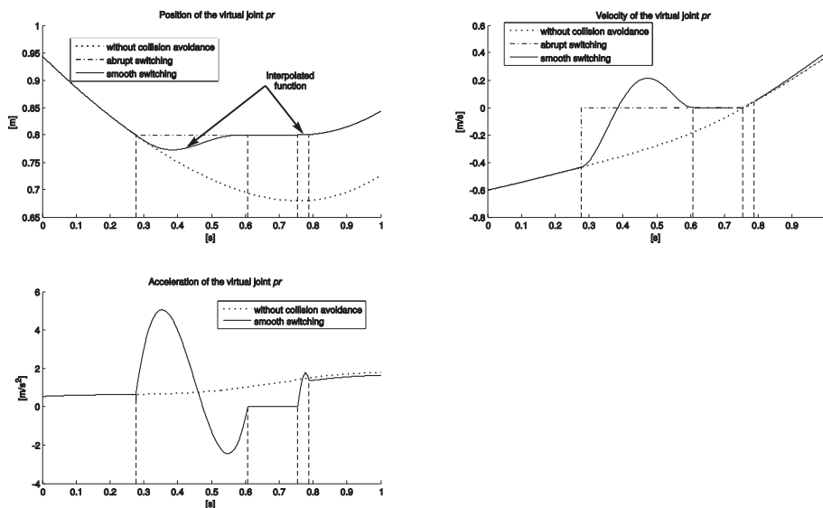
Figure 6. Resultant position, velocity and acceleration profiles for the virtual joint pr
