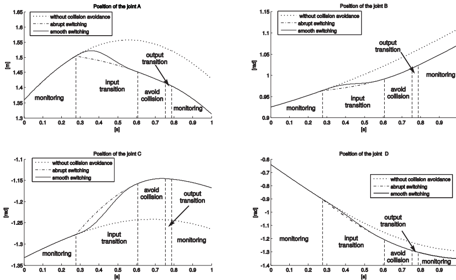
Figure 3. Position of the joints A , B , C and D
