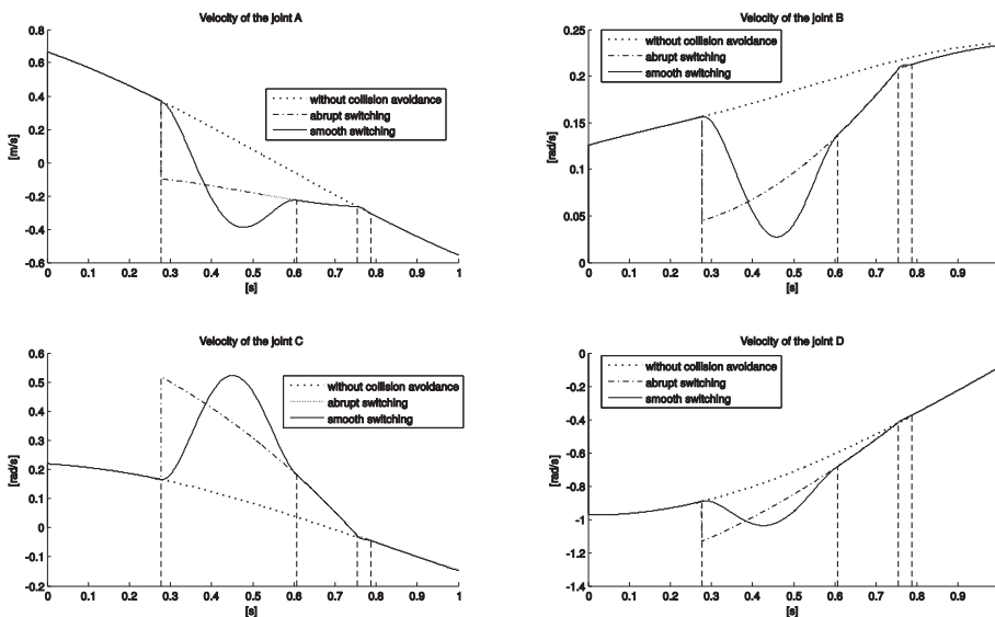
Figure 4. Velocities of the joints A , B , C and D
