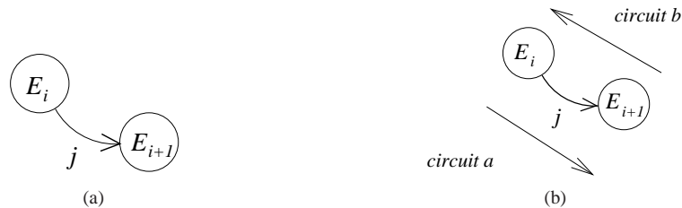
Figure 1. (a) Movement of link E_i relative to link E_{i+1} ; (b) Relation between joint j and the circuits a and b
