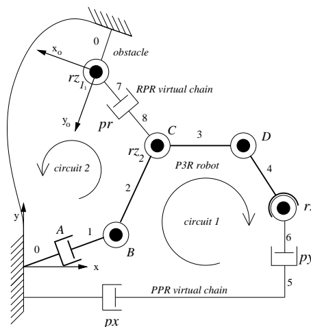
Figure 2. Complete kinematic chain
