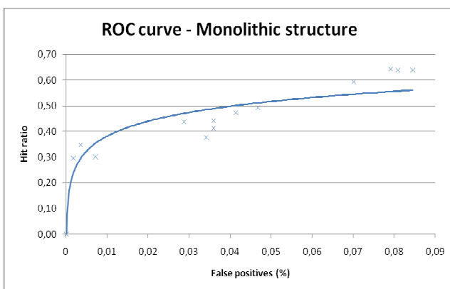
Figure 8. ROC curve obtained by Monolithic structure
