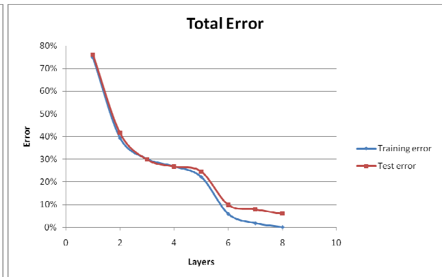
Figure 11. Total error with cascade structure.
