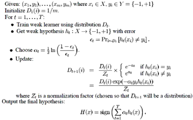
Figure 1. AdaBoost Algorithm (Freund, Schapire, 1999).
