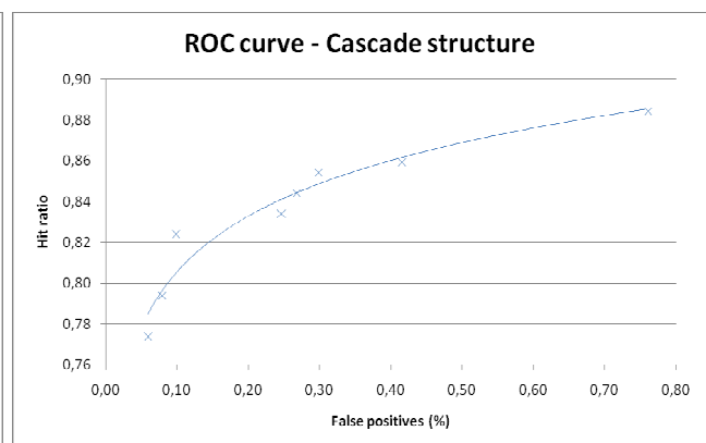
Figure 9. ROC curve obtained by Cascade structure
