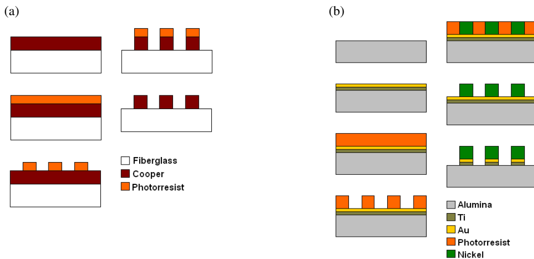
Figure 2. Microfabrication processes for: (a) Copper sensors, (b) Nickel sensors.
