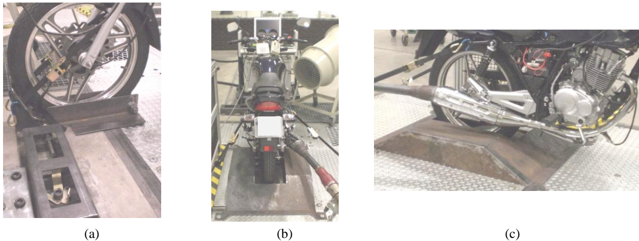
Figure 1. Mechanical assembly to fix the motorcycle at chassis dynamometer. (a) Front wheel (b) Side belt holders (c) Chassis dynamometer protection (Vinti, 2010).
