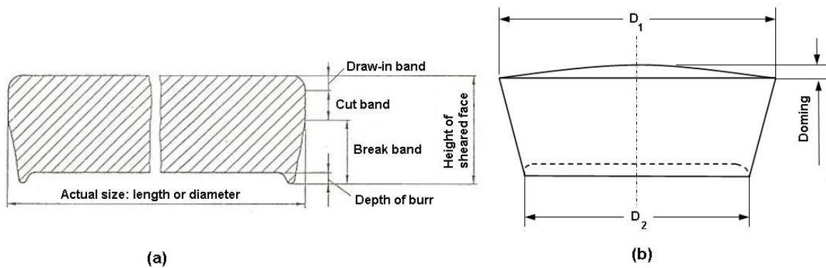
Figure 3. (a) Determination of the actual size of a stamped part (DIN6930, 1989). (b) Definition on form tolerance terms (Jana and Ong, 1989)
