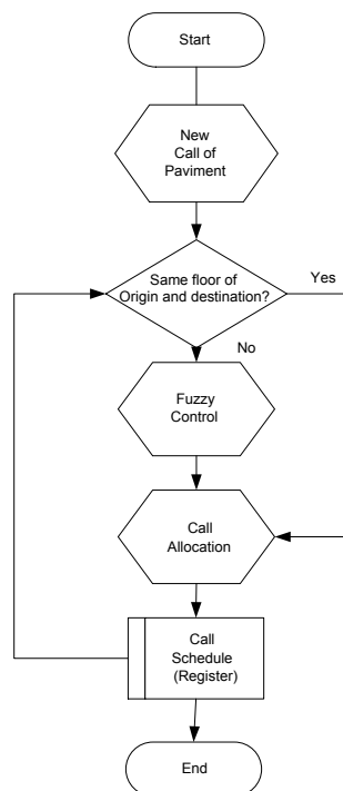
Figure 5 Sorting algorithm
