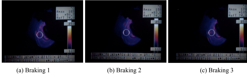
Figure 3.1-Thermographic images produced at velocity of 7,4 to 3,7 m/s and torque of 47 Nm (material B).
