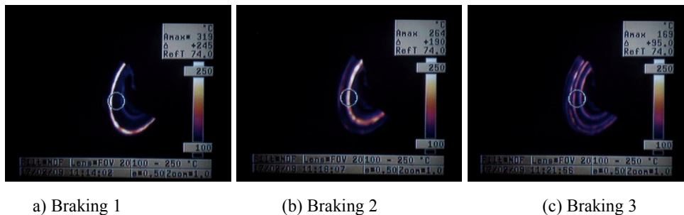
Figure 3.3-Thermographic images produced at velocity from 1,1 to 7,4 m/s and torque of 126 Nm (material B).
