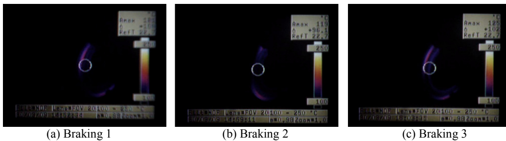
Figure 3.9 – Thermographic images produced at velocity of 16,6 to 13,8 m/s and torque of 47 Nm (material A).
