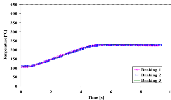
Figure 3.6 -Temperature curves measured by thermocouple (slipping velocity from 11,1 to 7,4 m/s, torque of 126 Nm and material A).
