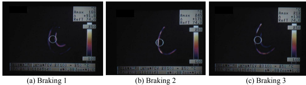
Figure 3.7 – Thermographic images produced at velocity of 16,6 to 13,8 m/s and torque of 47 Nm (material B).
