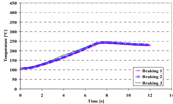
Figure 3.10 – Temperature curves measured by thermocouple (slipping velocity of 16,6 to 13,8 m/s, torque of 47 Nm and material A).
