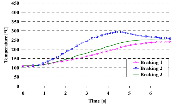
Figure 3.4-Temperature curves measured by thermocouple (slipping velocity from 11,1 to 7,4 m/s, torque of 126 Nm and material B).
