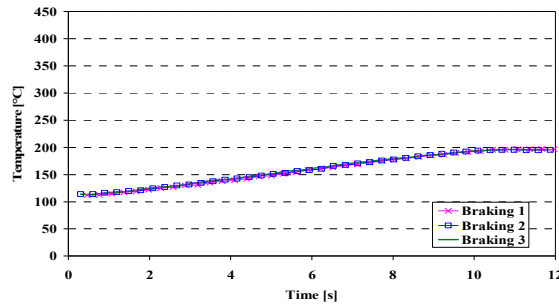
Figure 3.2 – Temperature curves measured by thermocouple (slipping velocity of 7,4 to 3,7 m/s, torque of 47 Nm and material B).
