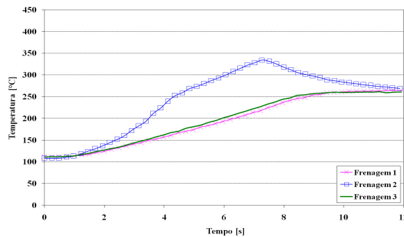
Figure 3.8 – Temperature curves measured by thermocouple (slipping velocity of 16,6 to 13,8 m/s, torque of 47 Nm and material B).
