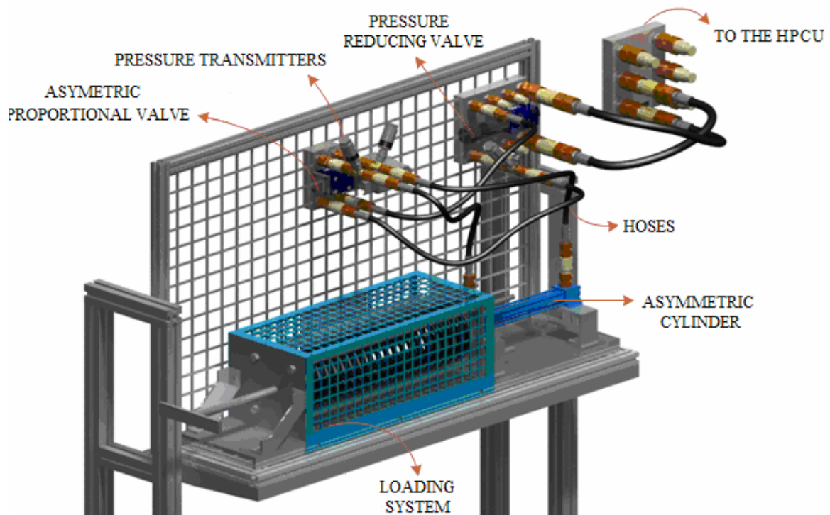
Figure 1. Work apparatus with a combination of asymmetric cylinder (AC) and asymmetric valve (AV).
