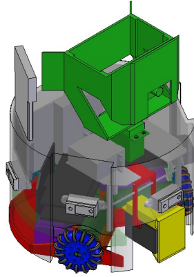
Figure 1. Axebot mobile robot
