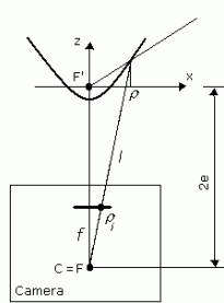
Figure 3. Catadioptric system
