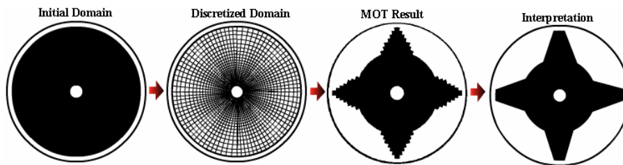
Figure 3 – Example of the TOM procedure applied to the design of an electrostatic micromotor.
