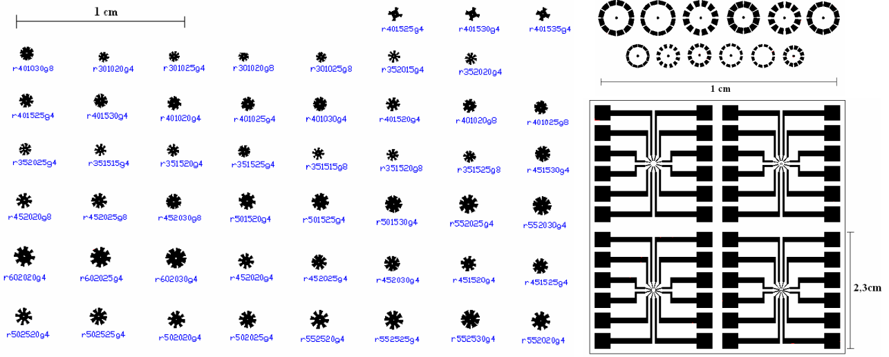
Figure 9 – Top view of the micromotor components mask: 50 rotors models (to the left); 12 stators models (in the superior right part); and 4 electric tracks models (in the inferior right part).
