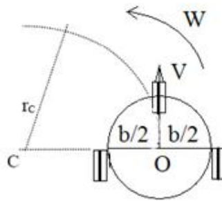
Figure 5. Direction for differential speed between the wheels.
