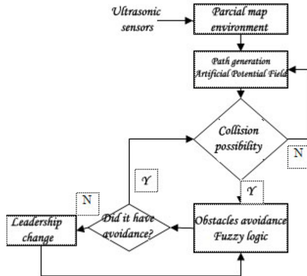
Figure 8. Flowchart of the control algorithm.
