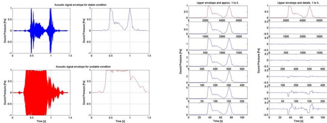
a) Envelope of stable and unstable vibration signals b) Six-level decomposition of a stable envelope signal
