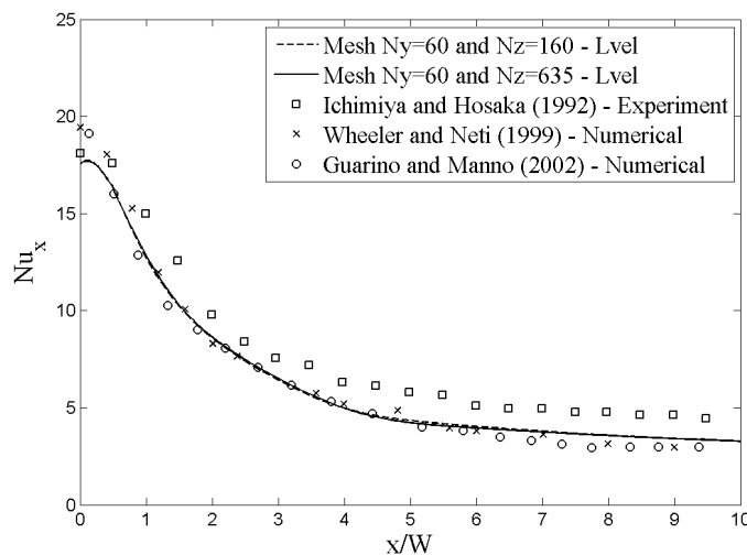
Figure 6. Local Nusselt number in two-dimensional confined jet.
