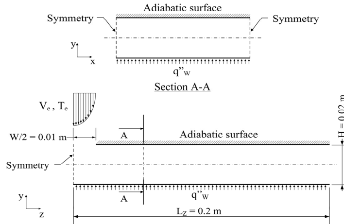
Figure 5. Duct configuration in two-dimensional confined jet.
