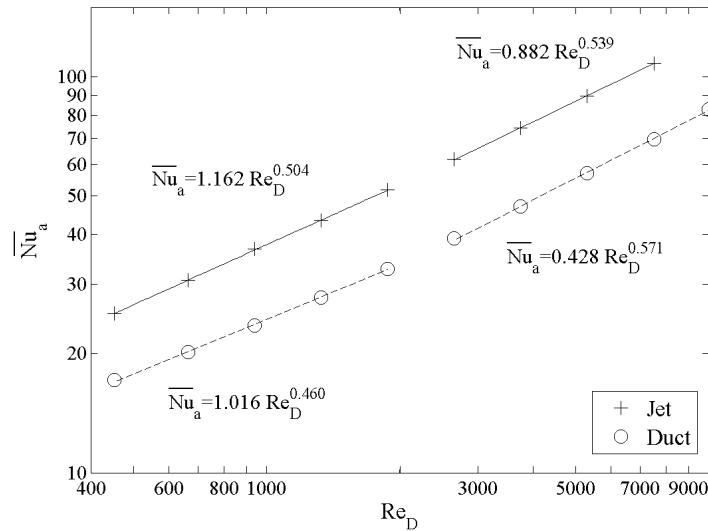
Figure 7. Average Nusselt number.
