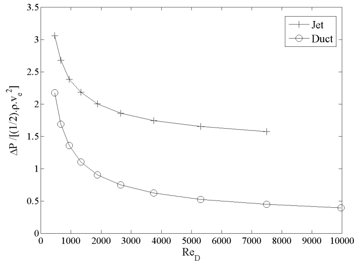
Figure 8. Dimensionless pressure drop – both configurations.
