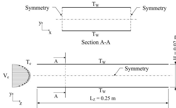
Figure 3. Dimensions and boundary conditions in channel flow.
