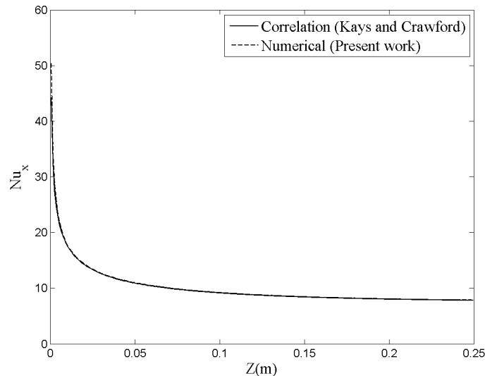
Figure 4. Local Nu_x in channel flow.
