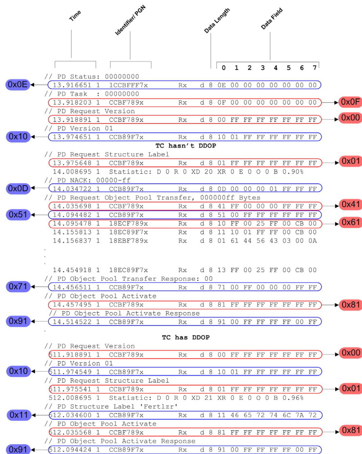
Figure 7. The CAN messages log of the initialization process among ECU1 and ECU4.
