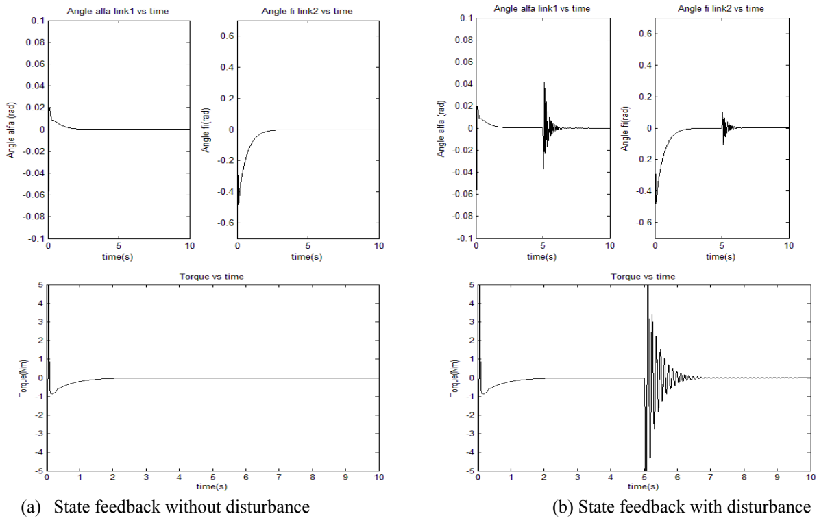
Figure 5. System controlled by state feedback.
