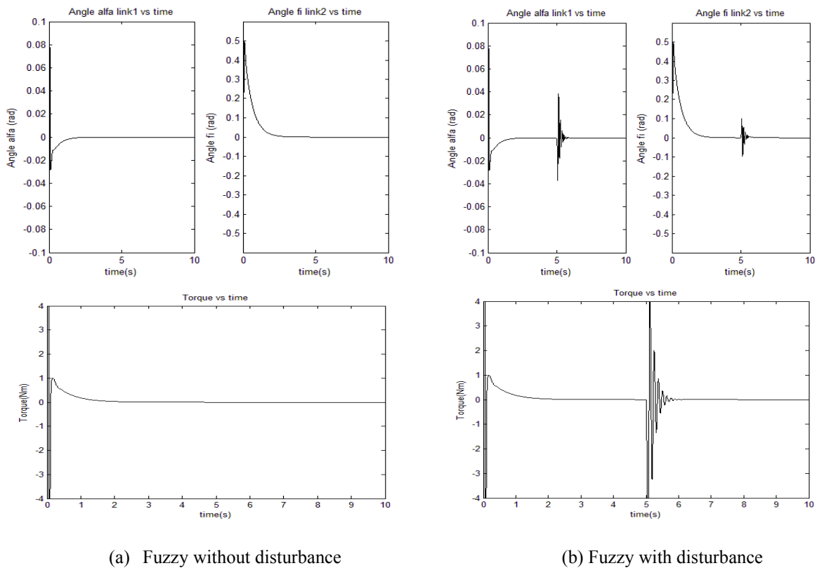
Figure 6. System with fuzzy controller optimized by ANFIS.
