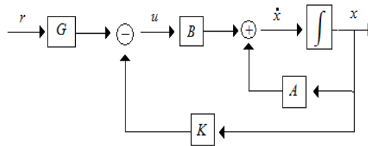
Figure 3. The block diagram of the state-feedback controller.
