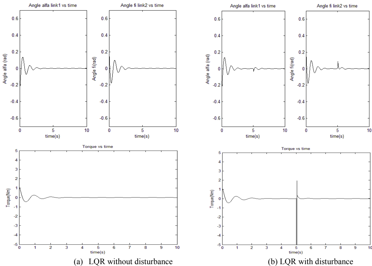
Figure 4. System controlled by LQR.
