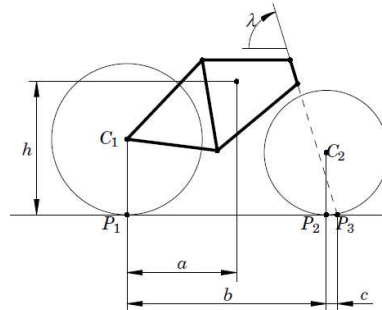
Figure 1. Parameters of geometric configuration for bicycle (Åström et al. , 2005)
