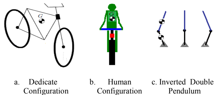
Figure 2. Model Approximation of Robot Cyclist.
