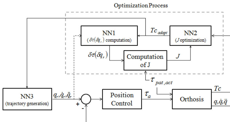
Figure 4. Structure of Neural Network-based system.
