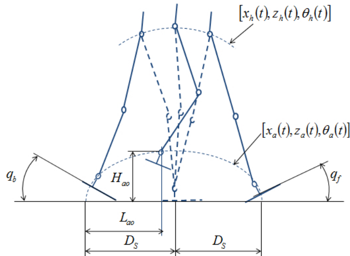
Figure 1. Biped robot model.
