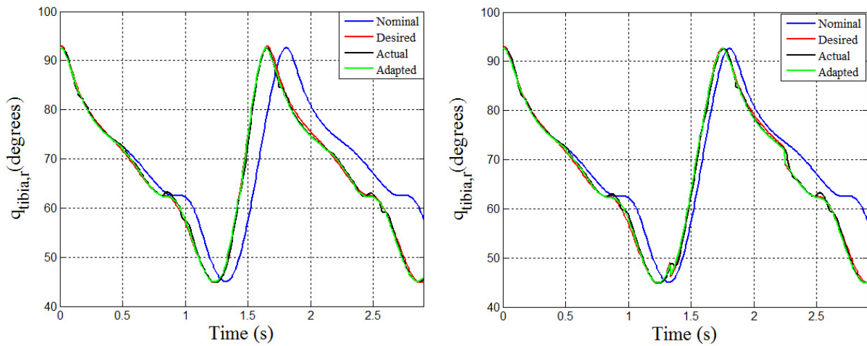
(a) Fix desired T_c for all time steps. (b) Desired T_c changing during walking. Figure 7. Nominal, patient desired, actual and adapted trajectories of the righth tibia, absolute angle.
