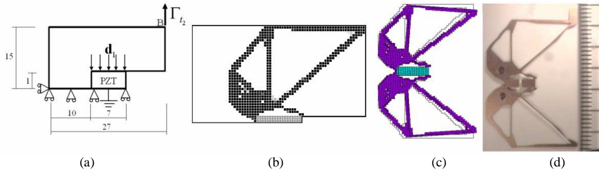
Figure 6. (a) initial design domain; (b) optimal topology; (c) deformed of the optimal topology and (d) manufactured actuator (1 division/mm).
