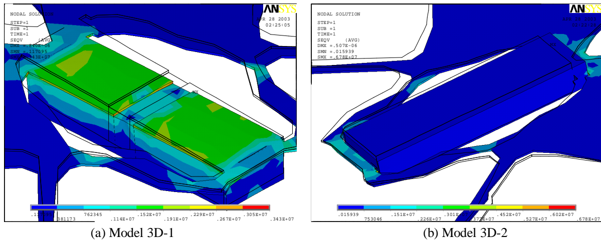
Figure 7. Von-Mises stress in Pa for the 3D models of manufactured prototype.
