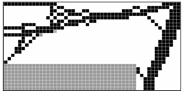
(b) w = 0,5 ; V^* = 20\% ; 1200 elements and filter turn off
