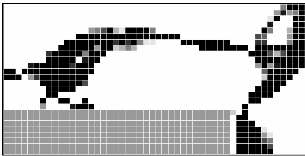
(c) w = 0,95 ; V^* = 20\% ; 1200 elements and filter turn off
