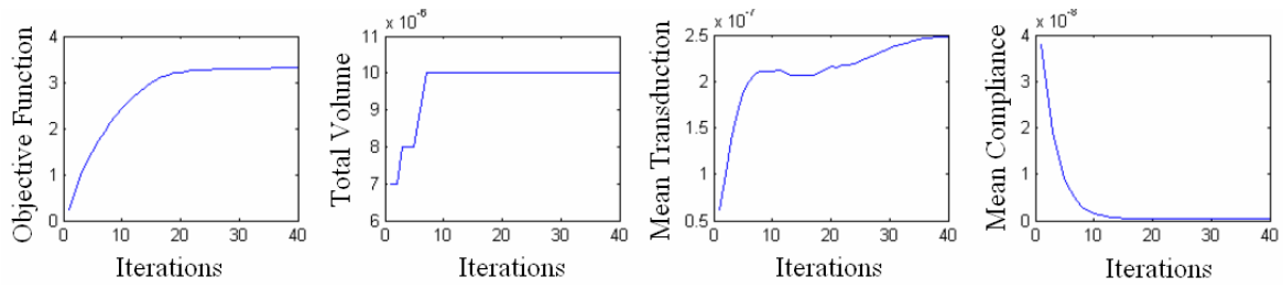
Figure 5. Graphs of convergence ( w = 0,5 ).
