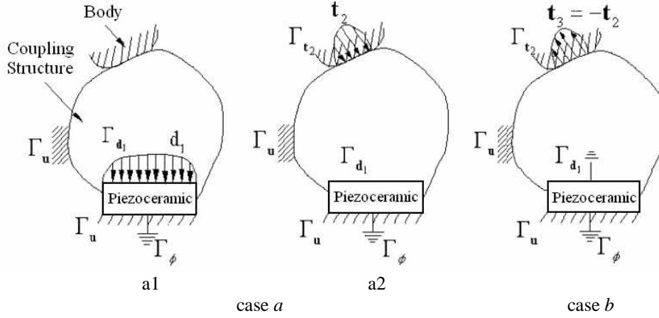
Figure 1. Load cases for calculation of the mean transduction (case a ) and mean compliance (case b ).
