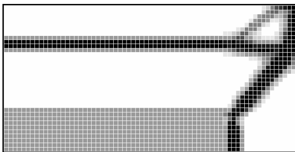
(e) w = 0,8 ; V^* = 15\% ; 2500 elements and filter turn on
