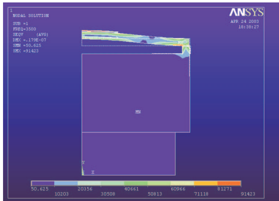
Figure 7. Von Mises stresses at resonance frequency of 10 mm mirror model.
