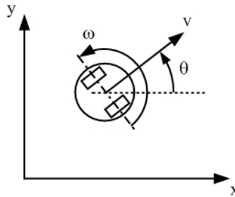
Figure 4: Description of the robot motion on Cartesian plane.
