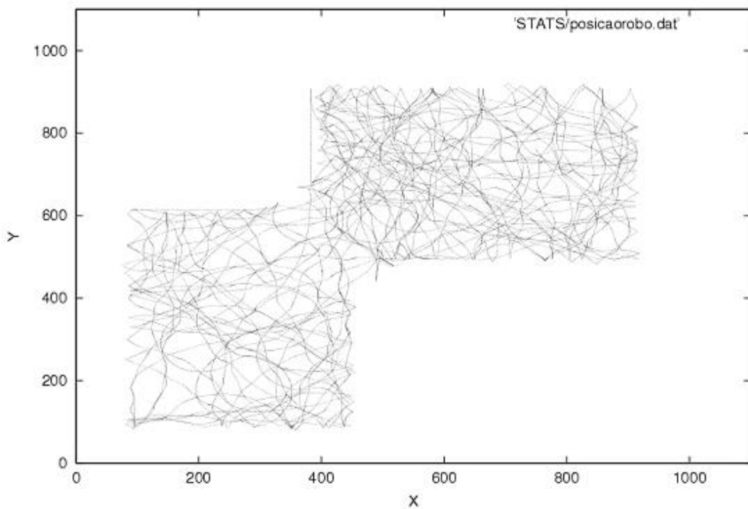
Figure 10: The KHEPERA robot trajectory using Lorenz system state variables x_2 and x_3 as control inputs. Position coordinates ( X and Y ) are expressed in millimeters.
