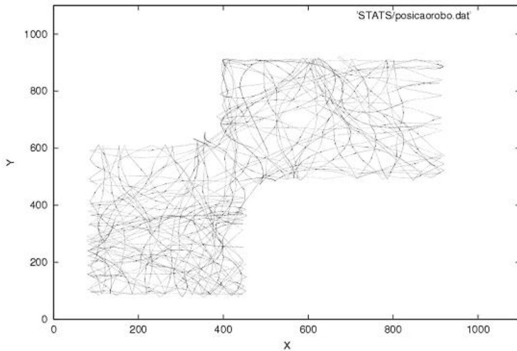
Figure 8: The KHEPERA robot trajectory using Lorenz system state variables x_1 and x_2 as control inputs. Position coordinates ( X and Y ) are expressed in millimeters.
