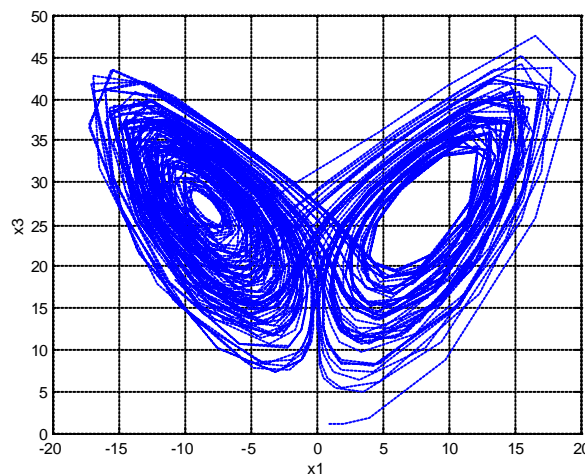
Figure 2: The x_1x_3 phase plan of Lorenz system.
