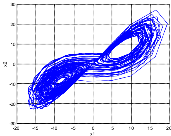
Figure 1: The x_1x_2 phase plan of Lorenz system.
