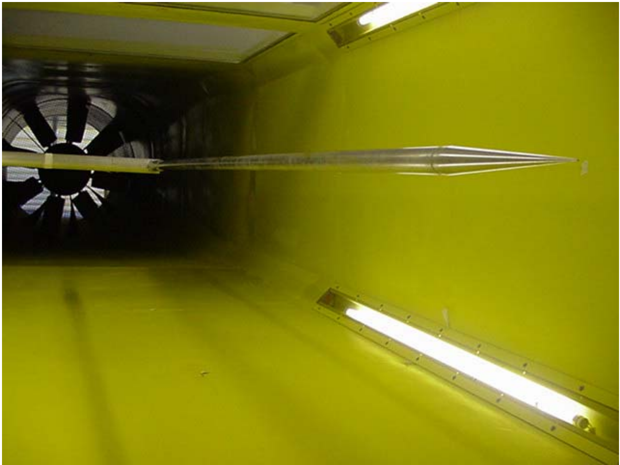
Figure 11. Long static tube inside the test section.
