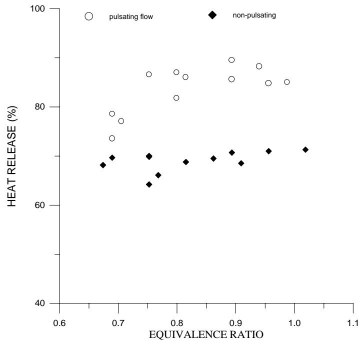
Figure 6. Percentage of the heat release to the water (fuel rate of the 0.15g/s)
