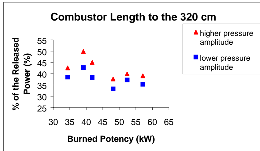
Figure 3: Percentage of heat transferred to water in a burned fixed section (Combustor length 320 cm).
