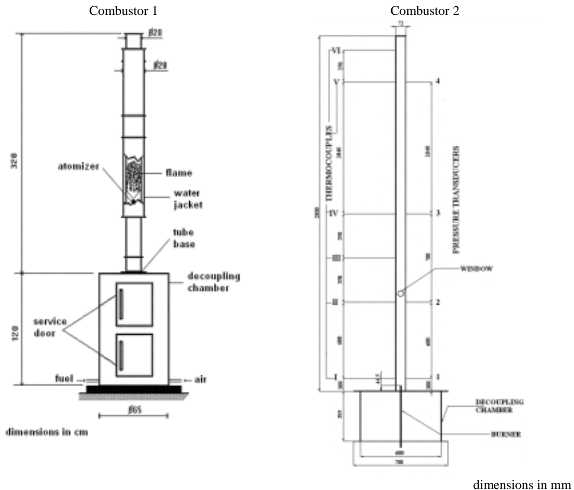
Figure 2 - Schematic diagrams for both Rijke tube combustors.
