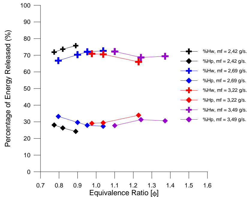
Figure 5 - Results of the energy balance for the testes described in Tab. (3) 1 .
