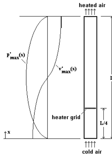
Figure 1 – Rijke Tube with open ends and the acoustic wave structure.
